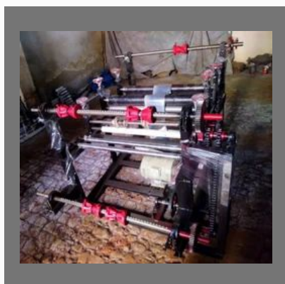
Paper Plate Lamination Machine
